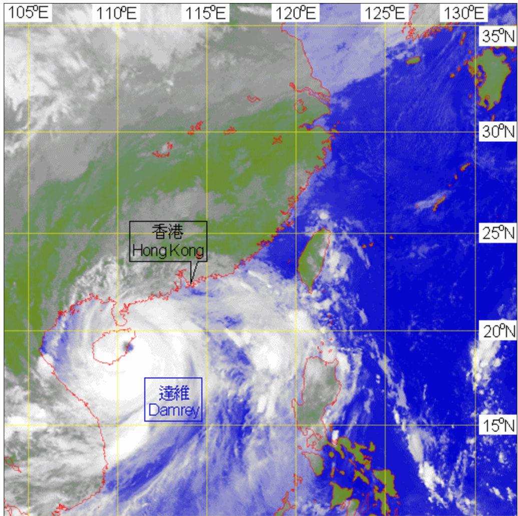
圖 3.3.3 達維在二零零五年九月二十六日約上午二時的紅外線衛星圖片。 [此衛星圖像接收自日本氣象廳的多用途輸送衛星-1R (MTSAT-1R)。] Figure 3.3.3 Infra-red imagery at around 2 a.m. on 26 September 2005 of Damrey. [The satellite imagery was originally captured with Multi-functional Transport Satellite-1R (MTSAT-1R) of Japan Meteorological Agency (JMA).]
