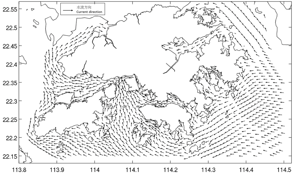
Trend of tidal current in Hong Kong waters during flood tide
