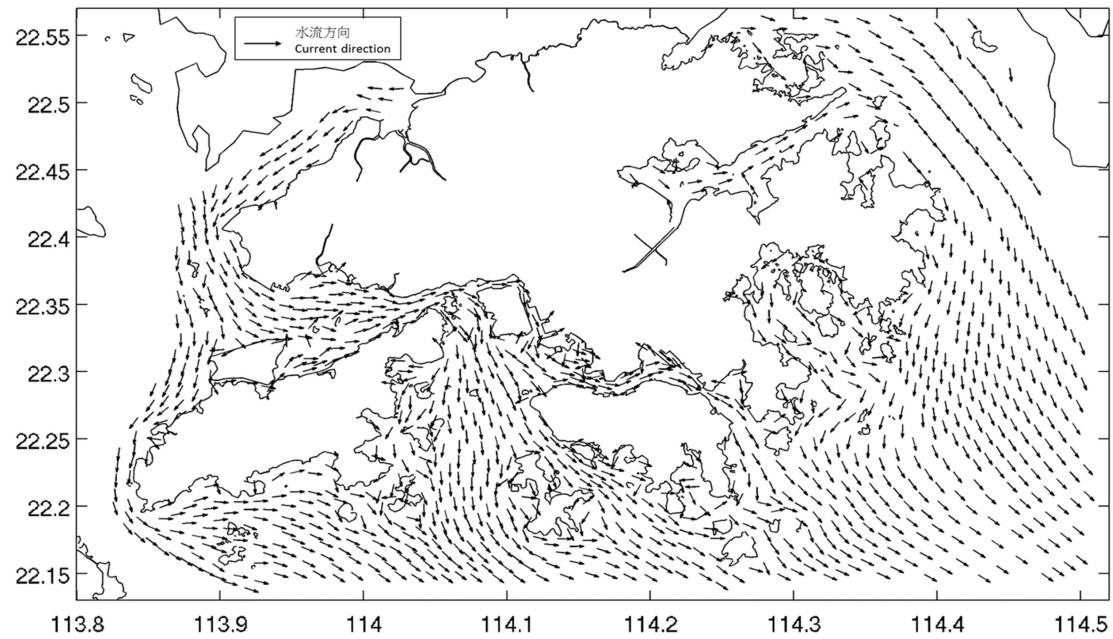
Trend of tidal current in Hong Kong waters during ebb tide
