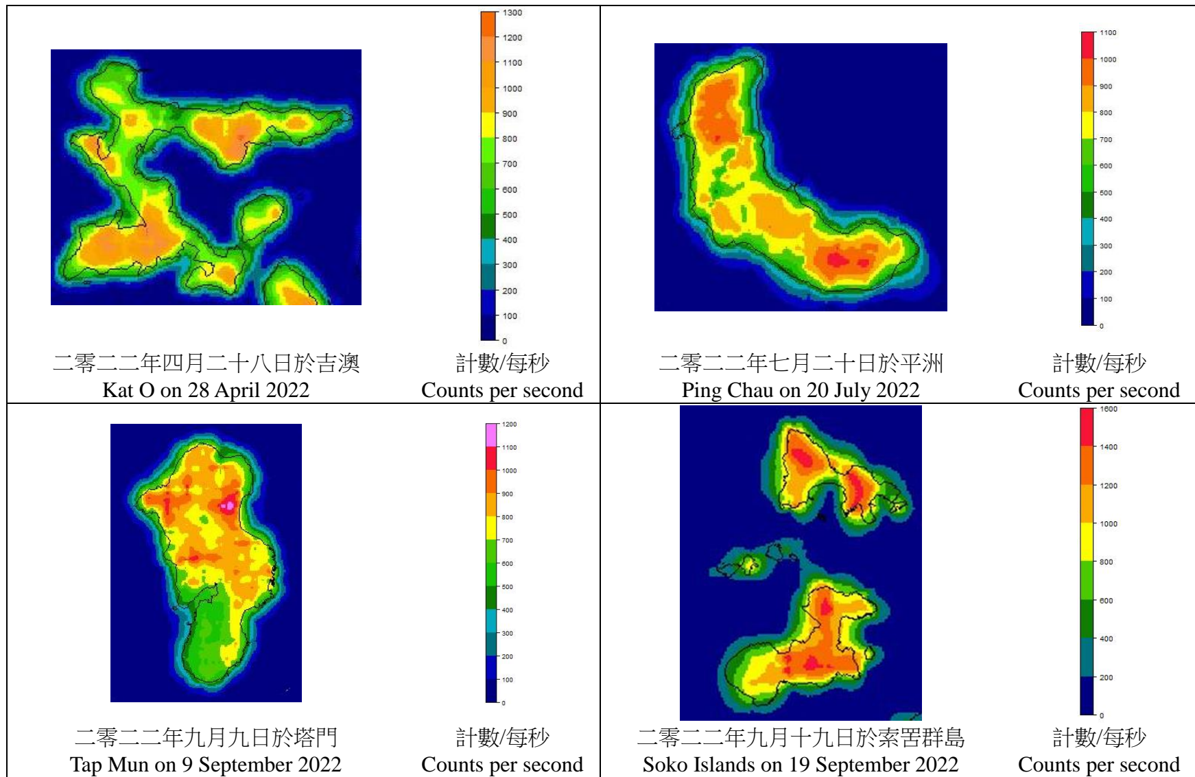
圖 4. 空中輻射監測系統在二零二二年分別於吉澳、平洲、塔門和索罟群島測量到的計數率(測量高度距離地面約一百米) Figure 4. Count rate over Kat O, Ping Chau, Tap Mun and Soko Islands respectively as measured by the Aerial Radiation Monitoring System in 2022 (at about 100 metres above the ground)
